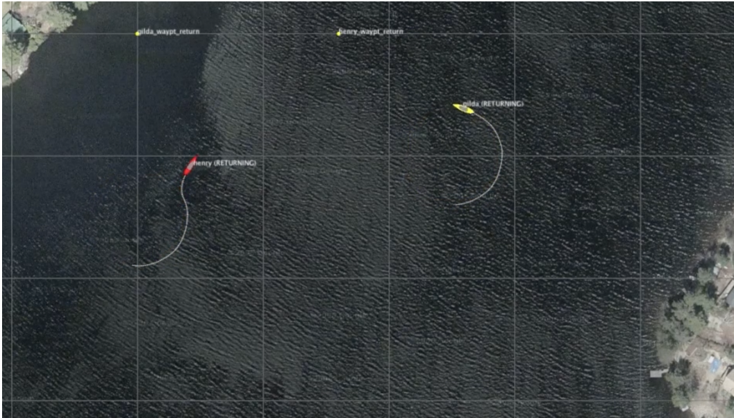
Figure 5: The Henry Gilda Refuel mission has two loitering vehicles. When the user commands the vehicles to return, they return to their starting point and station keep for 60 seconds and automatically re-deploy afterwards. As with the baseline mission, both vehicles have their own MOOS community, connected to a shoreside community, with the connections coordinated using the uField Toolbox utilities.
